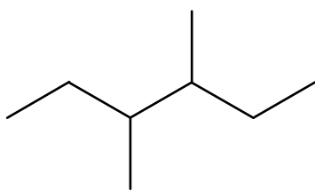
3,4-dimethyl-hexane
