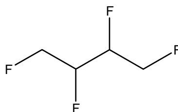
1,2,3,4-tetrafluoro-butane
