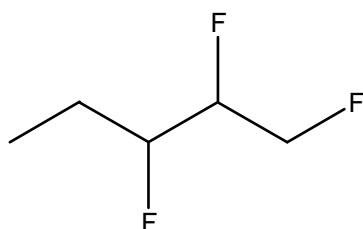
1,2,3-trifluoro-pentane
